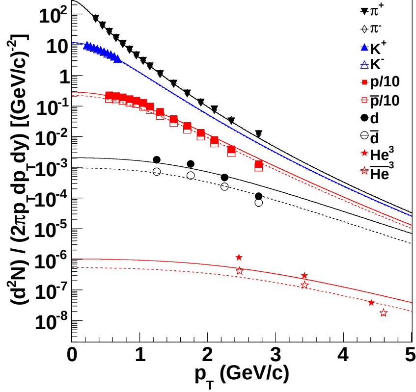
Figure 4.27: The transverse momentum spectra for identified particles including light nuclei ( d(\bar{d}) and {}^3\text{He}(\bar{{}^3\text{He}}) ) in minimum bias (0 – 80% centrality) Au+Au collisions at \sqrt{s_{NN}} = 200 GeV. The symbols represent experiment data points. The curves represent the TBW fit for the hadrons. The curves for the light nuclei are the TBW prediction using parameters from the fit to other hadrons.
