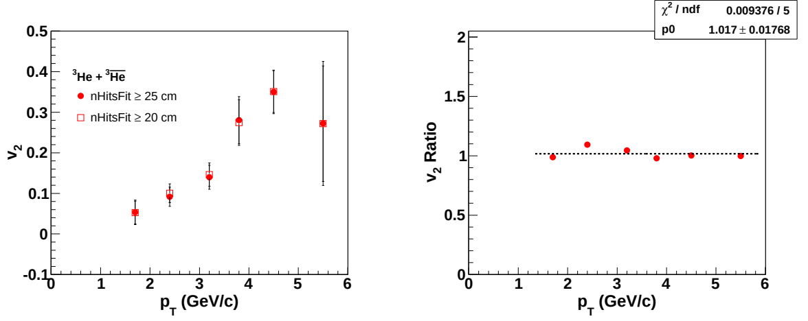
Figure 4.17: Left panel: Variation of v_2 for {}^3\text{He} + {}^3\overline{\text{He}} with the variation of n\text{HitsFit} cut in minimum bias Au+Au collisions at \sqrt{s_{NN}} = 200 GeV. Right panel: Ratio of measured v_2 for {}^3\text{He} + {}^3\overline{\text{He}} with n\text{HitsFit} \geq 25 and n\text{HitsFit} \geq 20 .
