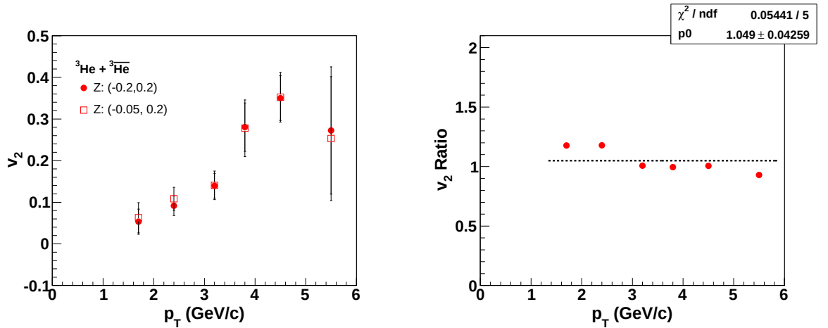
Figure 4.18: Left panel: Variation of v_2 for {}^3\text{He} + {}^3\overline{\text{He}} with the variation of Z range to identify {}^3\text{He} candidates in minimum bias Au+Au collisions at \sqrt{s_{NN}} = 200 GeV. Right panel: Ratio of measured v_2 for {}^3\text{He} + {}^3\overline{\text{He}} with |Z({}^3\text{He})| < 0.2 and -0.05 < Z({}^3\text{He}) < 0.2 .
