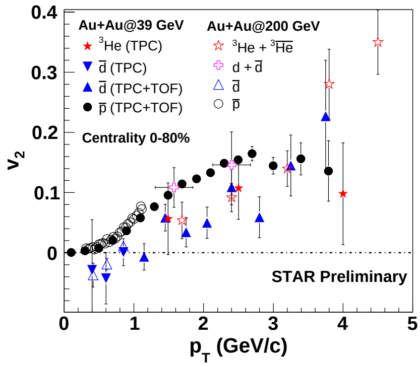
Figure 4.30: v_2 as a function of p_T for d(\bar{d}) and ^3\text{He}(\bar{^3\text{He}}) from 0-80% of the collision centrality in Au+Au collisions at \sqrt{s_{NN}} = 200 GeV and 39 GeV. v_2 of \bar{p} at the two energies are shown for the comparison [18, 19].
