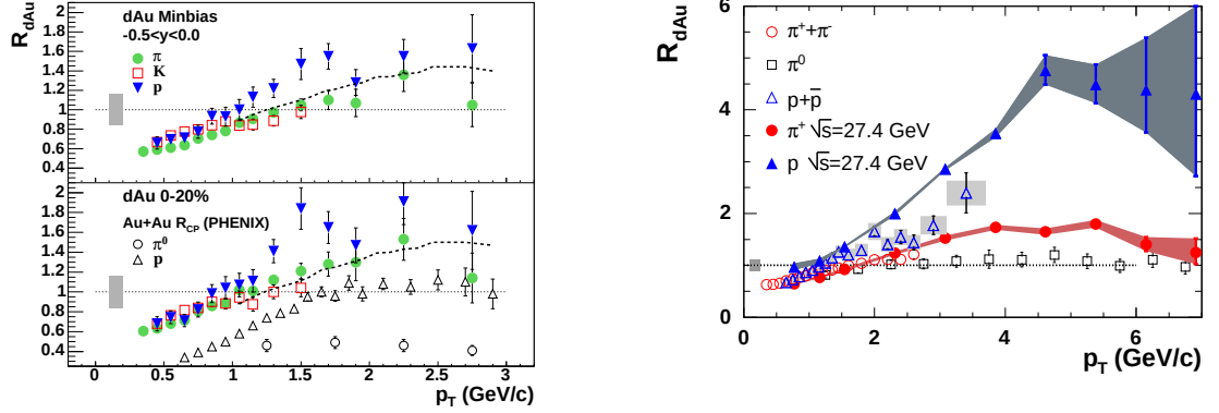
Figure 1.22: Nuclear modification factors for the identified particles from d +Au collisions at \sqrt{s_{NN}} = 200 GeV, measured by the STAR (left) and PHENIX (right) experiments at RHIC [54, 55]. Nuclear modification factors calculated from the per-beam nucleon cross sections reported for \sqrt{s_{NN}} = 27.4 GeV p + A collisions are also shown for the comparison (right) [52].
