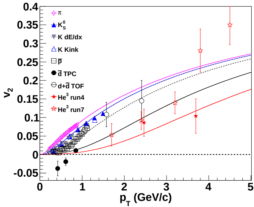
Figure 4.28: v_2 as a function of p_T for identified particles including light nuclei ( d(\bar{d}) and {}^3He(\bar{{}^3He}) ) in minimum bias (0 – 80% centrality) Au+Au collisions at \sqrt{s_{NN}} = 200 GeV. The symbols represent experiment data points. The curves represent the TBW fit for the hadrons. The curves for the light nuclei are the TBW prediction using parameters from the fit to other hadrons.
