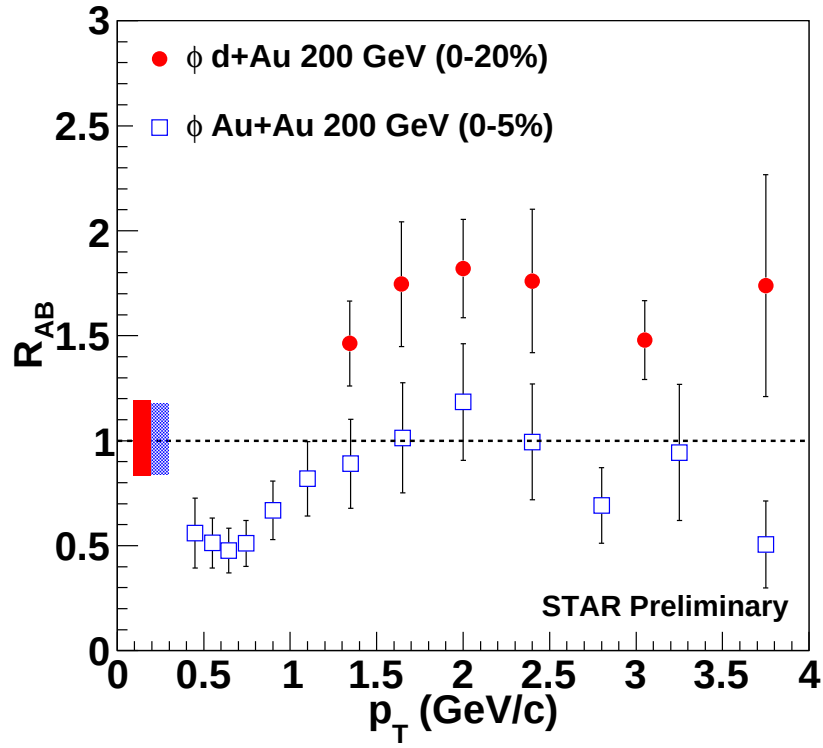
Figure 3.11: p_T dependence of the nuclear modification factor R_{AB} for \phi meson in 0-20% d+Au and 0-5% Au+Au [16] collisions at \sqrt{s_{NN}} = 200 GeV. Errors are statistical only. The normalization uncertainties for 0-20% d+Au and 0-5% Au+Au collisions are shown in red and blue rectangular bands, respectively.
