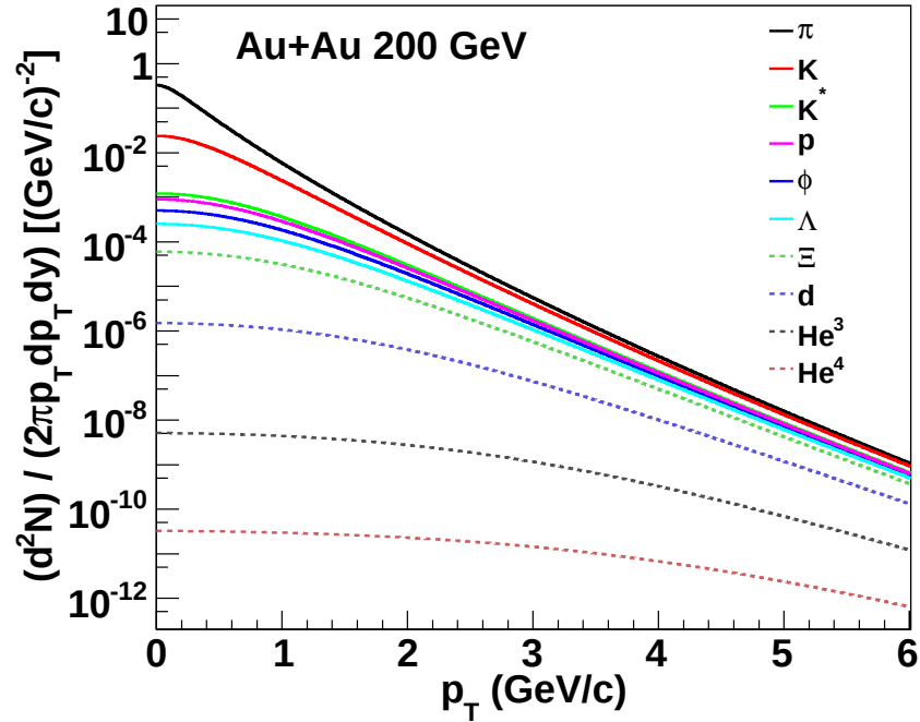
Figure 5.5: The transverse momentum spectra for identified particles including light nuclei ( d(\bar{d}) , {}^3He(\bar{{}^3He) , and {}^4He(\bar{{}^4He) ) in 0-10% Au+Au collisions at \sqrt{s_{NN}} = 200 GeV. The spectra for light nuclei are predicted by TBW model using parameters from the fit to other hadrons.
