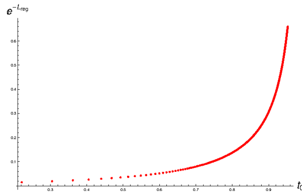
Figure 3.4: Plot of e^{-L_{reg}} as a function t_0 for the soliton solution.
