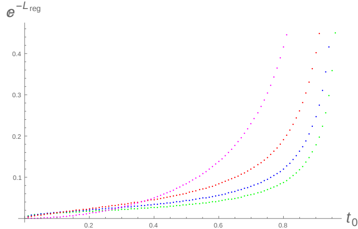
Figure 3.1: Plot of e^{-L_{reg}} vs t_0 for different values of p . Magenta, blue and green are for p = 9/10, 1/5 and 1/7 respectively. For p = 1/3 , the numerical and analytical results coincide. The behaviour is shown above in red.
