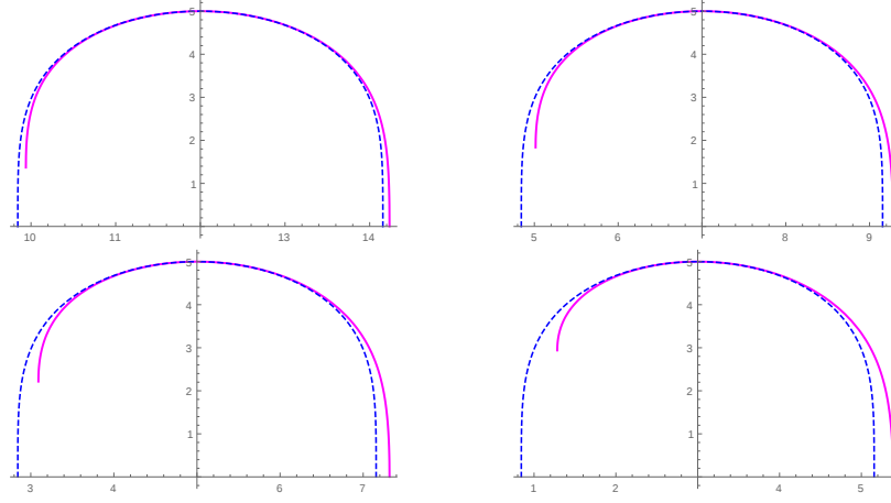
Figure 4.4: In these three plots we take, z_* = 5 and (a) r_0 = 12 , (b) r_0 = 7 , (c) r_0 = 5 , (d) r_0 = 3 .
