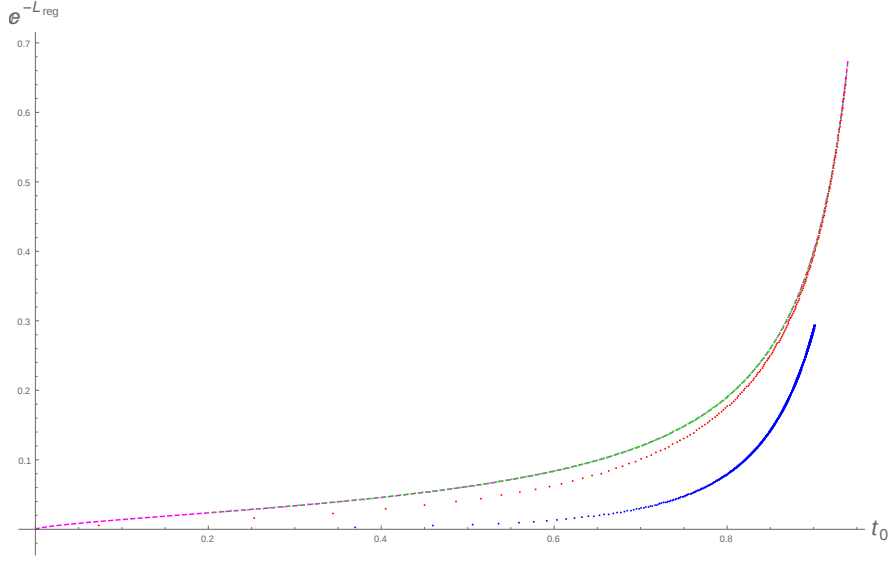
Figure 3.3: Plot of e^{-L_{reg}} vs t_0 for AdS_7 Kasner soliton. Blue, red and green curves are for z_0 = .5, 1 and 10 respectively. For comparison, we also showed, in magenta, e^{-L_{reg}} for pure AdS_7 Kasner solution.
