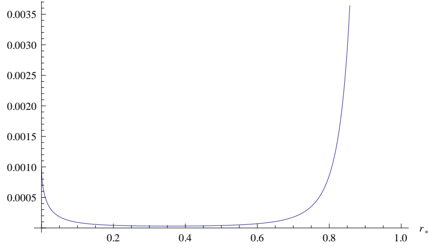
Figure 4.2: Here we plot \langle O(-x, r_*) O(x, r_*) \rangle vs. r_* for p = \frac{1}{3} with m = 5 .
