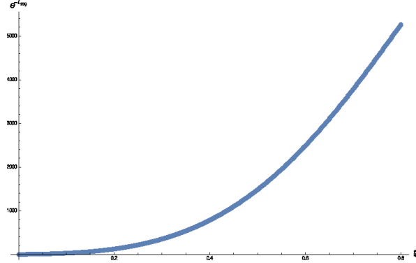
Figure 3.2: Plot of e^{-L_{reg}} as a function of t_0 for p_1 = p_2 = \frac{1}{2} , p_3 = 0 non-vacuum AdS-Kasner solution. As the space-like surface at t_0 is pushed towards t = 0 , the correlator vanishes.
