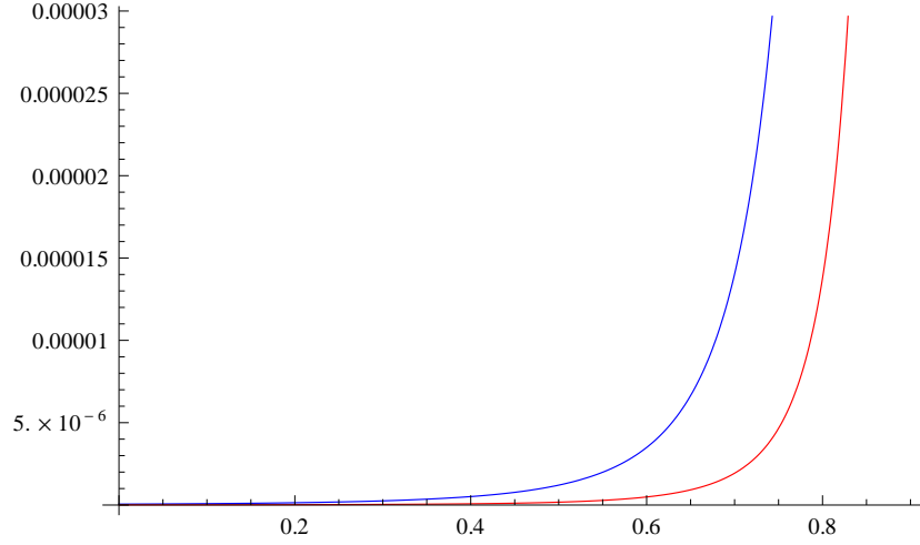
Figure 4.1: They are plots of f(\bar{r}_0) vs. \bar{r}_0 . Blue and red graphs are for p = -\frac{1}{4} and p = -\frac{1}{6} respectively, m = 5 .
