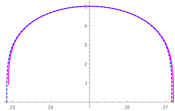
Figure 4.3: Here we plot the cross-section of the extremal surface in z - r plane. The magenta curve is the surface described by 4.39 whereas dashed blue curve shows that of a pure AdS. In this plot, z_* = 5 and r_0 = 25 .
