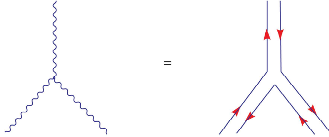
Figure 3.3. 3-pt vertex \sim \frac{1}{g_{YM}^2}
