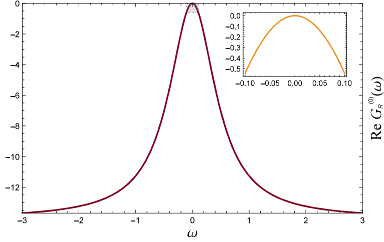
Figure 6.2. Real part of G_R^{(0)}(\omega) with \mu_* = 5
