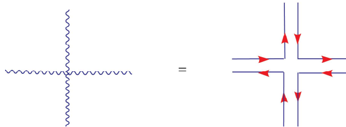
Figure 3.4. 4-pt vertex \sim \frac{1}{g_{YM}^2}
