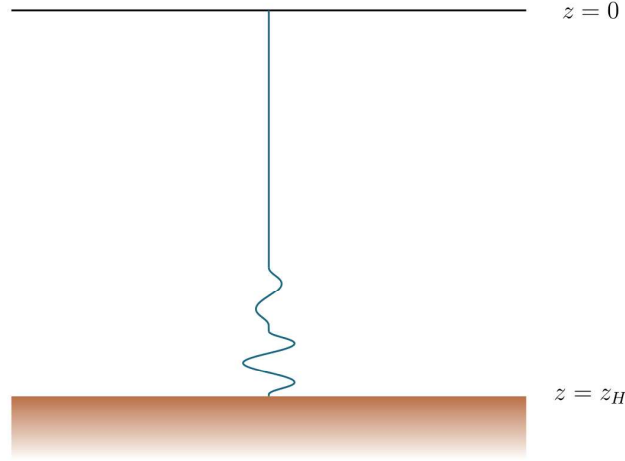
Figure 6.1. Gravity set up describing Brownian motion
